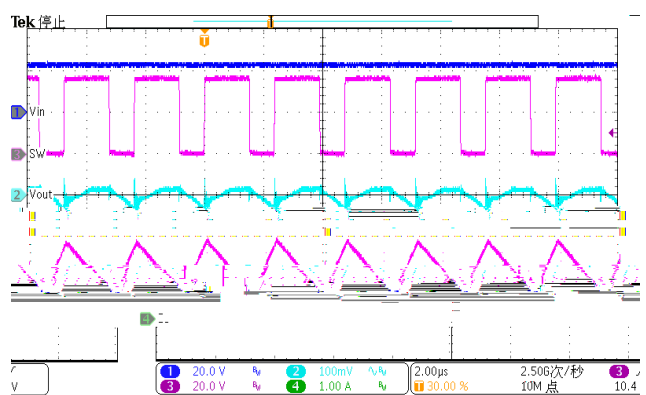
Figure 36. steady-state (Iload=2A)
