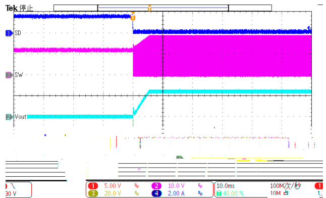
Figure 34. Shutdown remove
